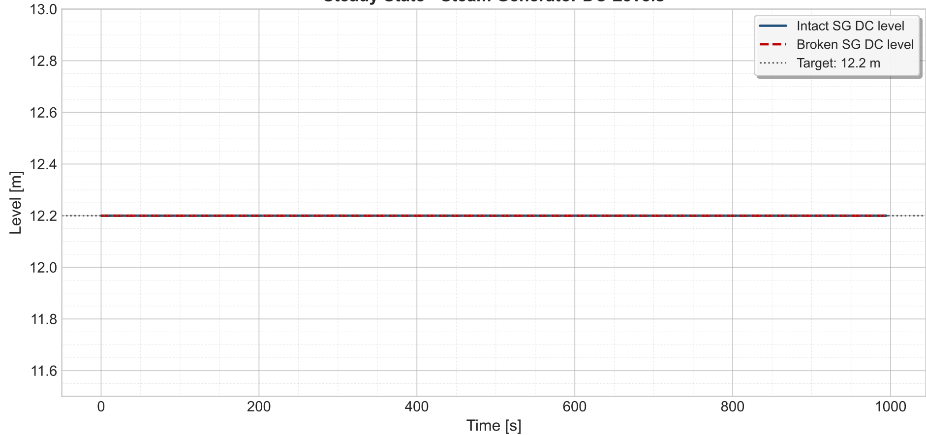
Steady State - Steam Generator DC Levels
